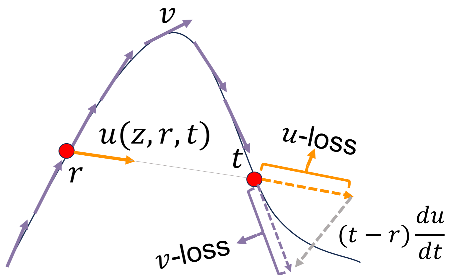
(b) Mean Flow vs. Our Improved Mean Flow
