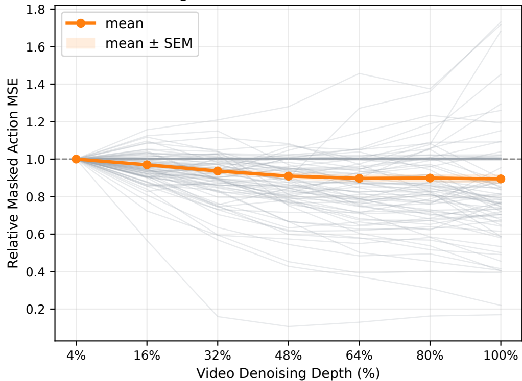
Coarse Segments: Relative Masked Action MSE
