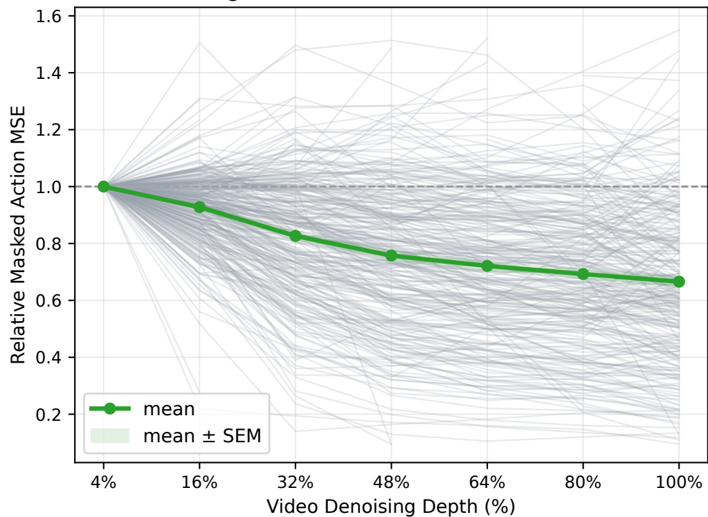
Fine Segments: Relative Masked Action MSE
