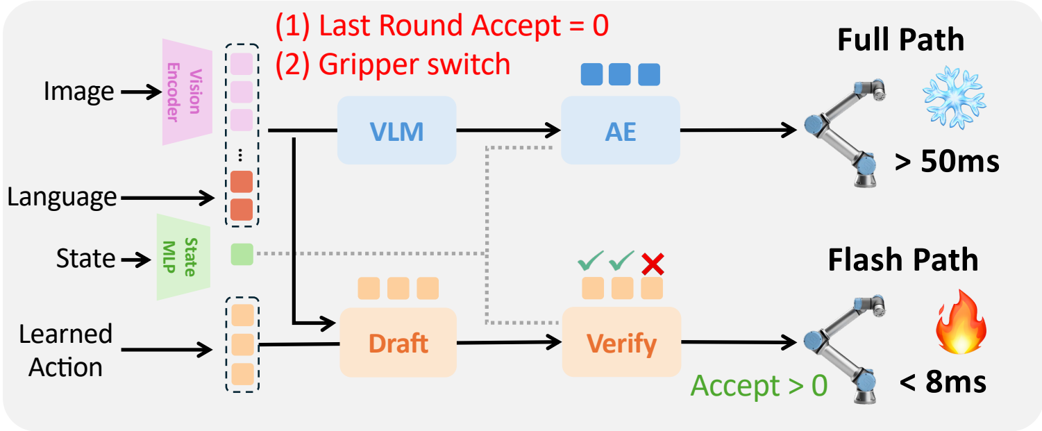
(a) Realtime-VLA FLASH Framework
